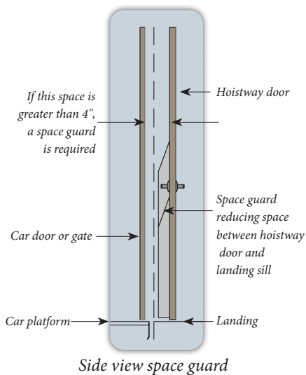
Plastic space guard at 36"
